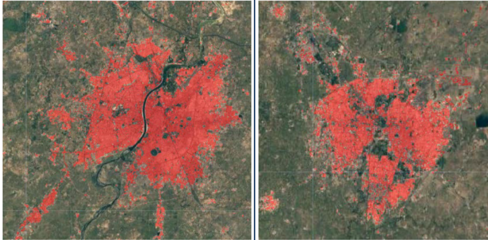
Figure 8: source is Goldblatt et al. (2018)
