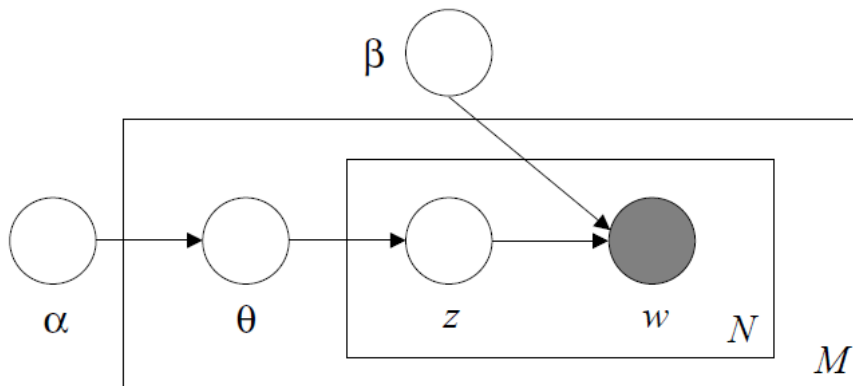
Figure 4: source is Blei et al. (2003)
