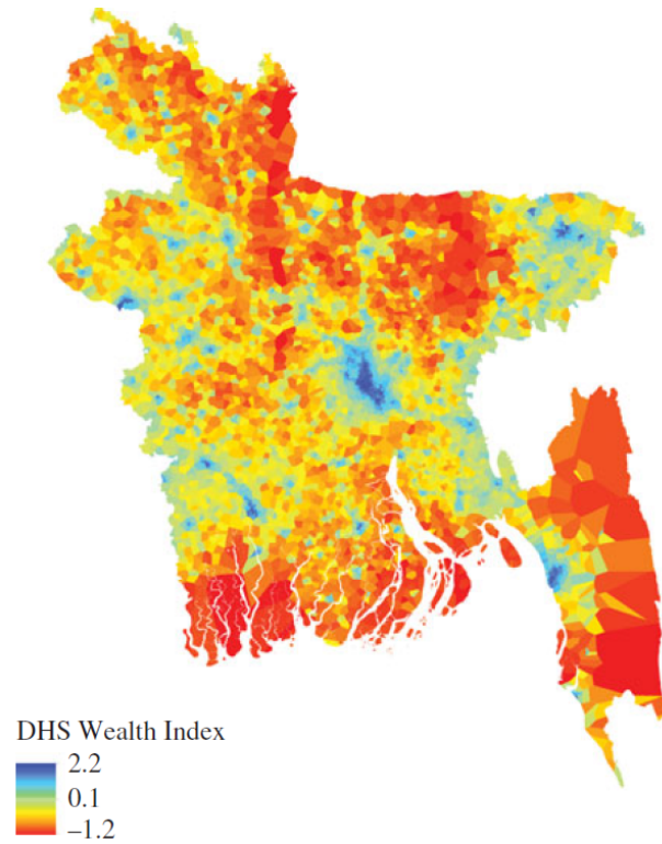
Figure 7: source is Steele et al. (2017)
