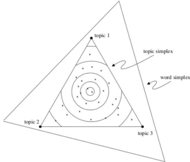
Figure 5: source is Blei et al. (2003)
